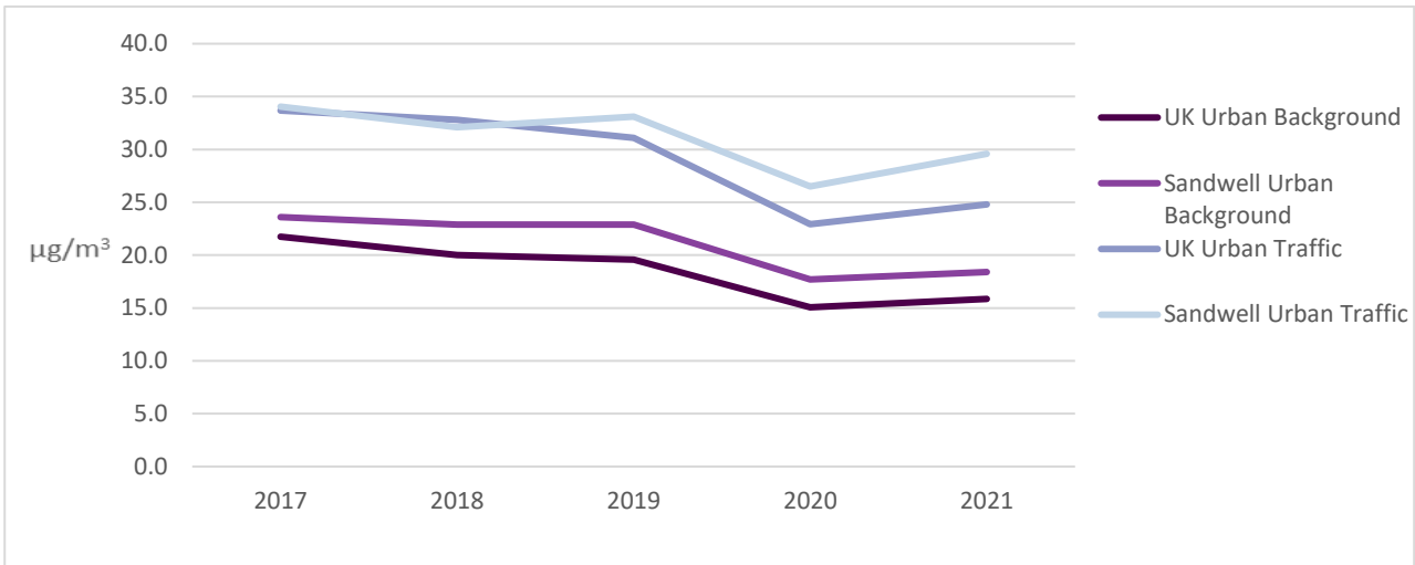
Figure 1.1- Comparison between the UK and Sandwell's Annual Mean NO 2 at Urban Background and Urban Traffic Sites
