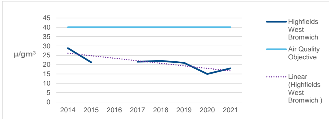
Figure 3. 3- Annual Mean Nitrogen Dioxide Concentrations at Highfields, West Bromwich 2014 -2021
