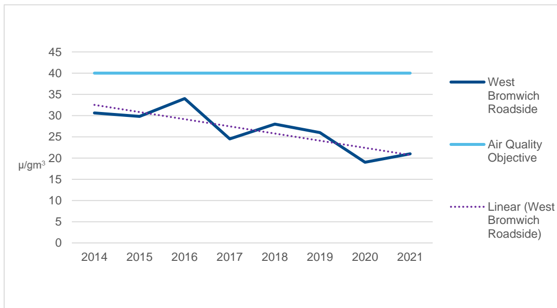
Figure 3. 1 - Annual Mean Nitrogen Dioxide Concentrations at West Bromwich Roadside 2014- 2021
