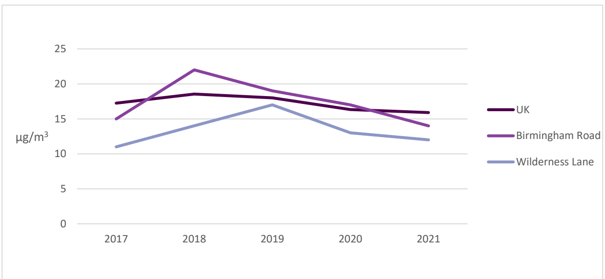
Figure 1.2 - Comparison between the UK and Sandwell's Annual Mean PM10 concentrations at Urban Traffic Sites
