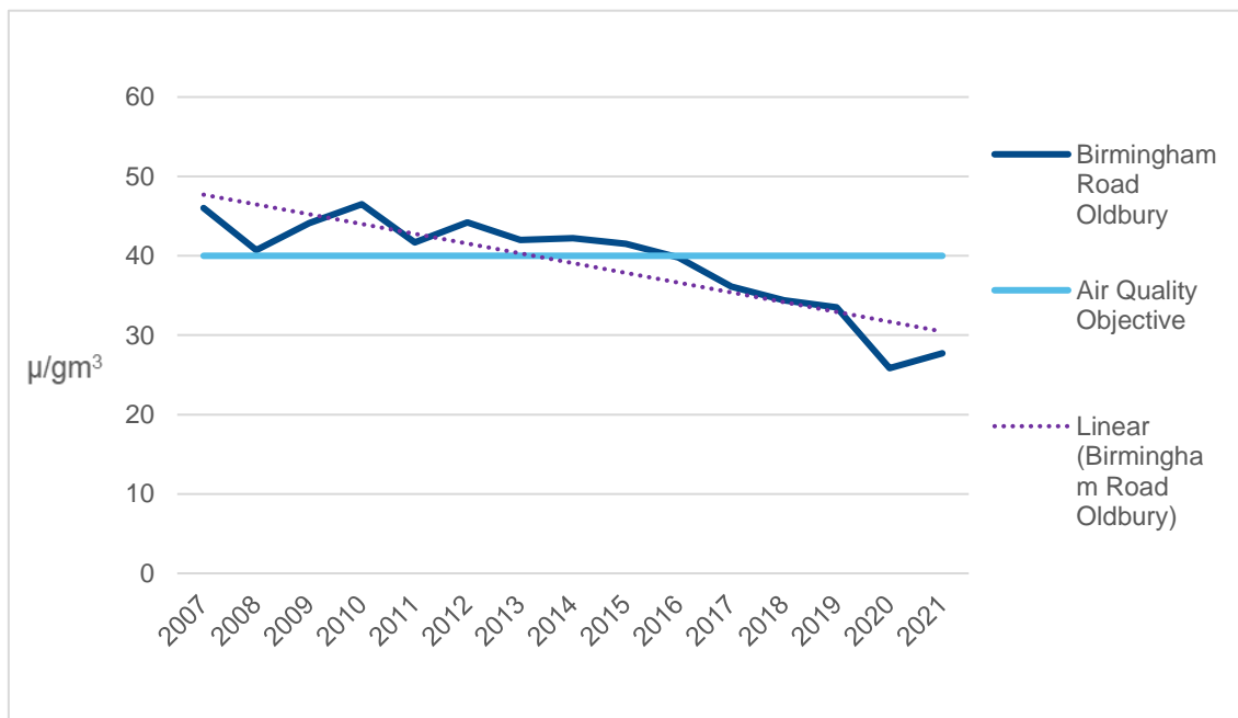
Figure 3. 2 - Annual Mean Nitrogen Dioxide Concentrations at Birmingham Road, Oldbury 2007- 2021
