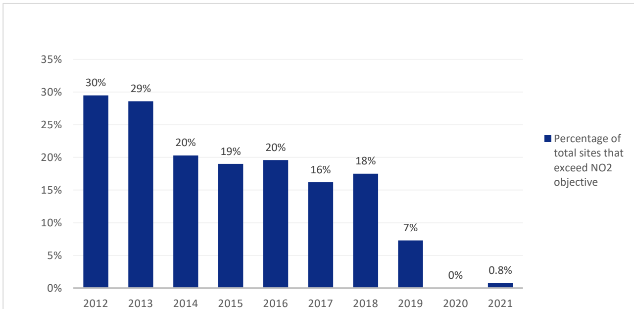
Figure 3. 6 - Percentage of NO 2 diffusion tube sites in Sandwell that exceed National Air Quality Objective
