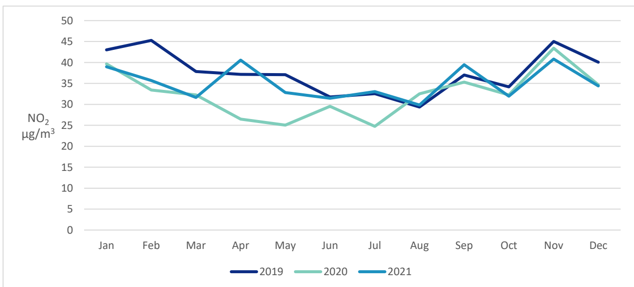
Figure 3. 7 - Comparison between Monthly NO 2 Averages in Sandwell 2019, 2020 and 2021
