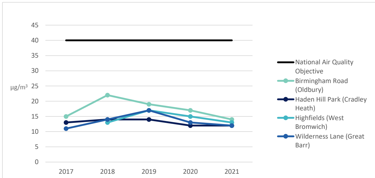
Figure 3. 8 - Trends in Annual Mean PM10 Concentrations at Continuous Monitoring Stations in Sandwell 2017-2021
